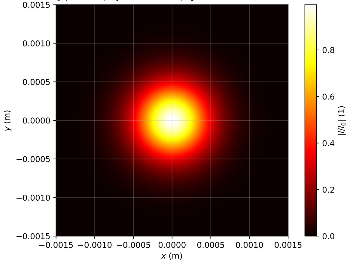
Intensity profile I(x, y, z = 0.955m)/I_0 , \text{Pin}=0.4\text{Pcr} , artificial time
